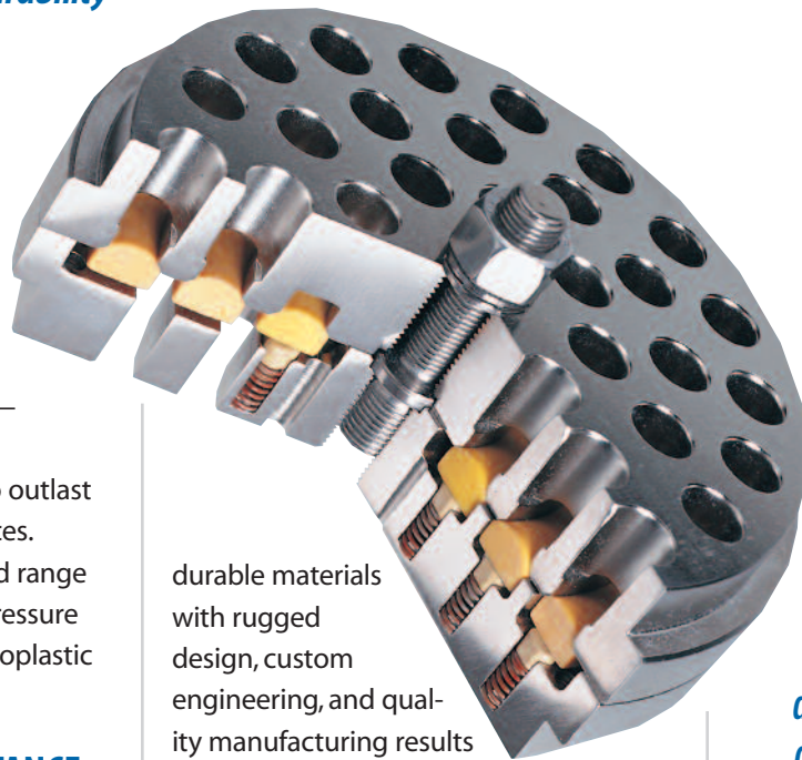
Conventional valve
