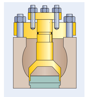
HSR assembly
